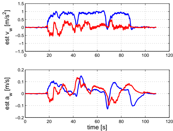
Fig. 16. Experiment 3 (with control rotation): Estimated intentional walker velocities and accelerations in the frame (X_w, Y_w) — x components in blue, y components in red
